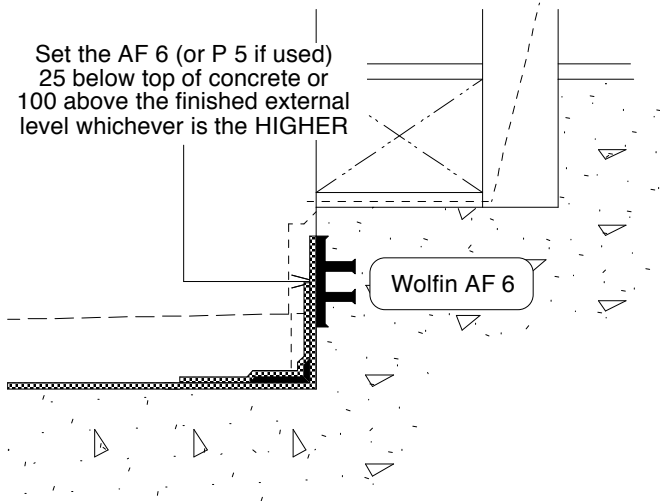
TYPICAL at CONCRETE SETDOWN or HOB Refer detail 1.01 for general notes
