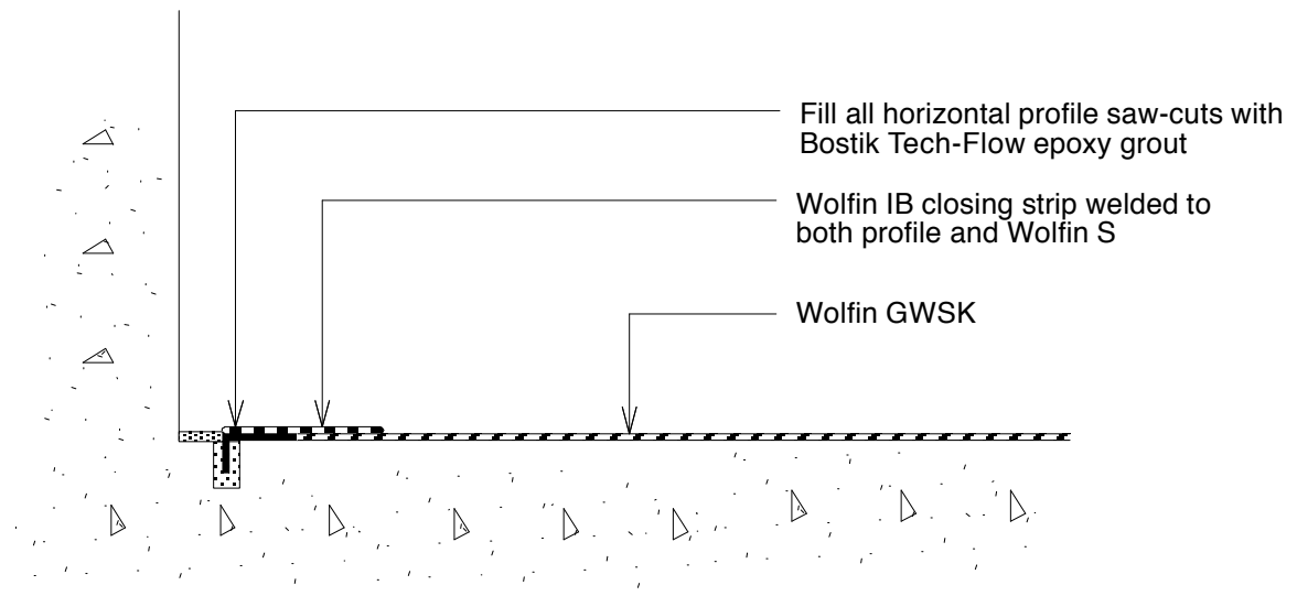
HORIZONTAL TERMINATION DETAIL
