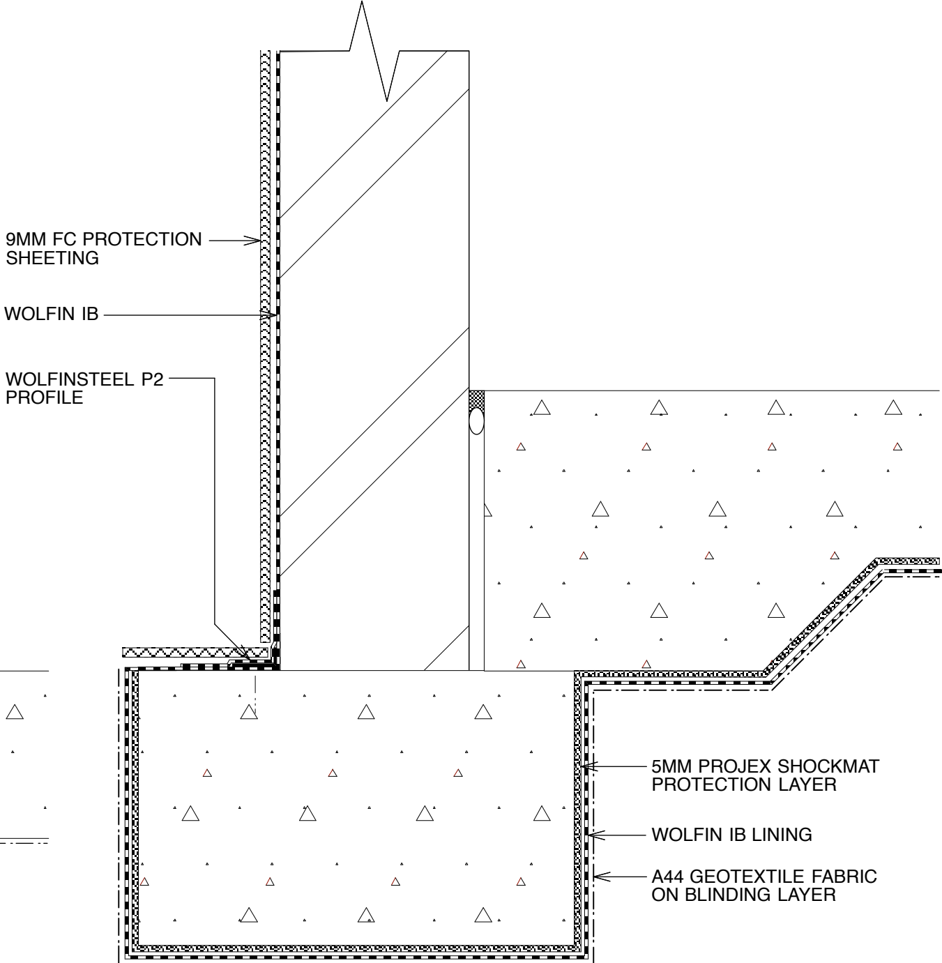
SECTION: BASEMENT WALL ON FOOTING - INTERNAL SLAB
