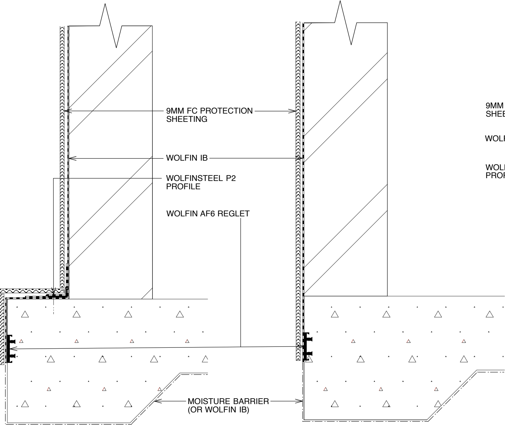
SECTION: BASEMENT WALL ON SLAB JUNCTION DETAIL - OFFSET
